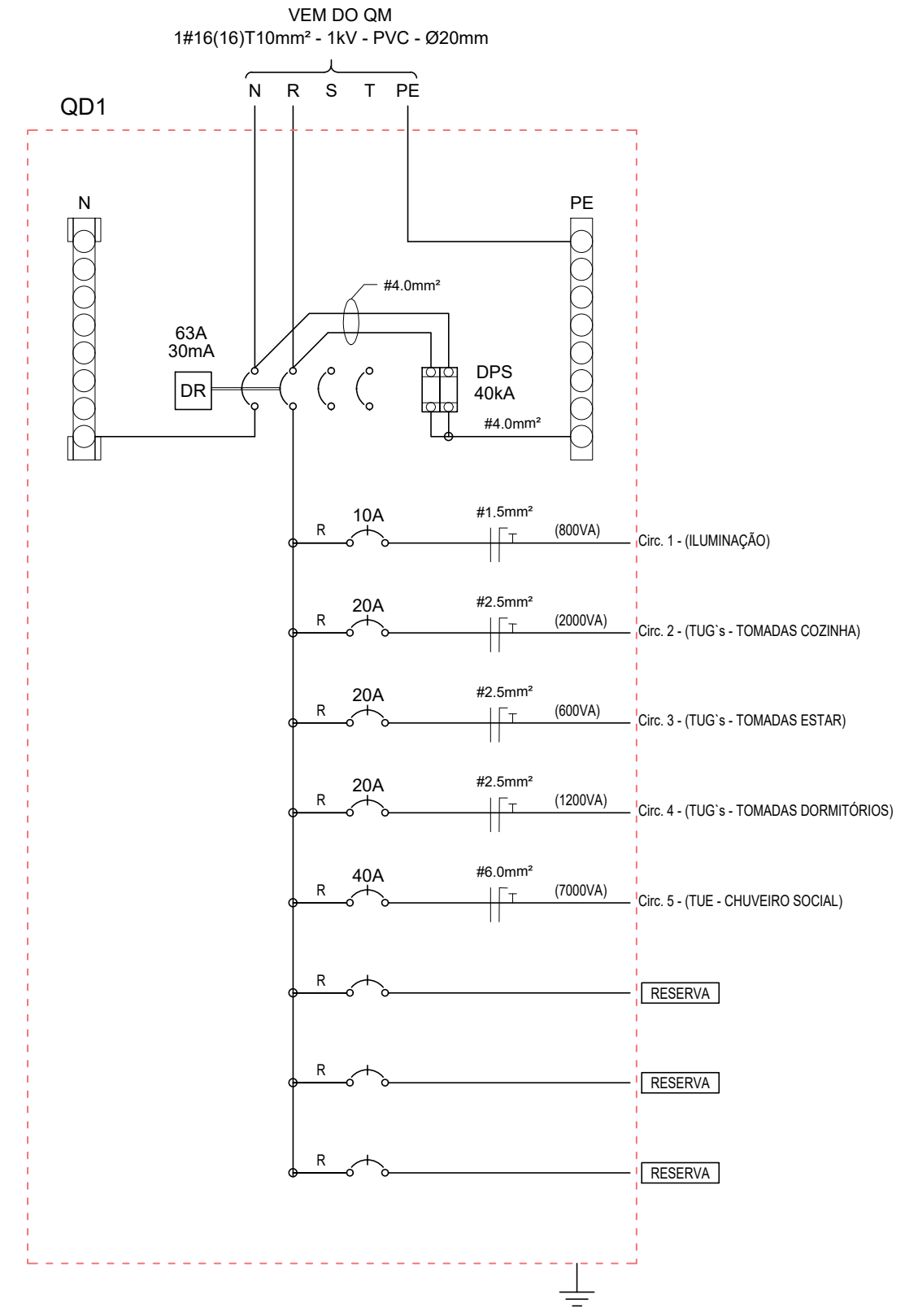
DIAGRAMA MULTIFILAR
