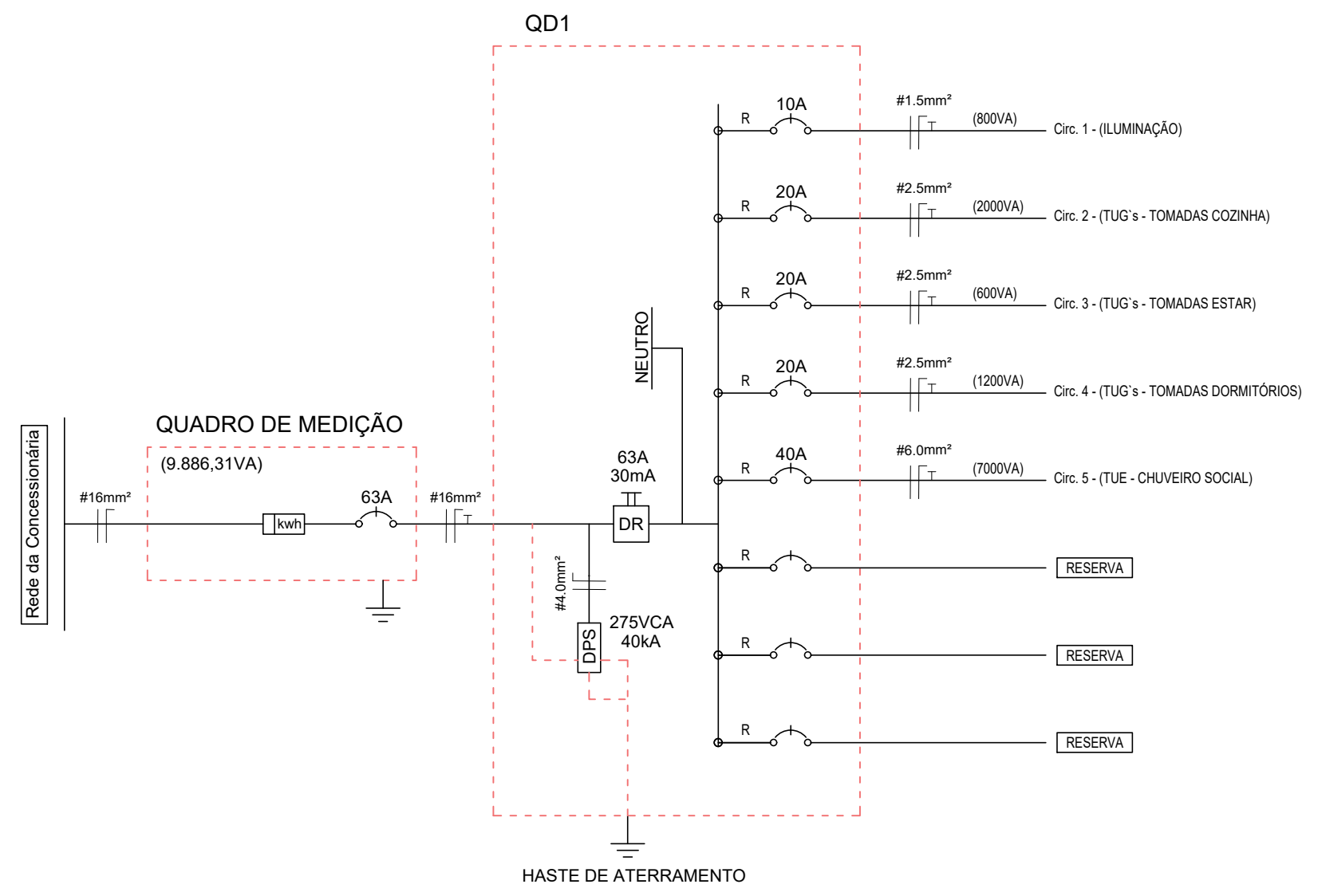
DIAGRAMA UNIFILAR
